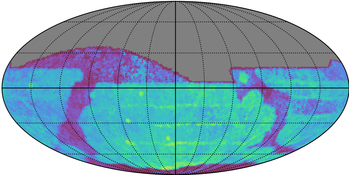
too_combined_no_nss_s10.0_v3.4_10yrs All sky z band: Median Season Length
