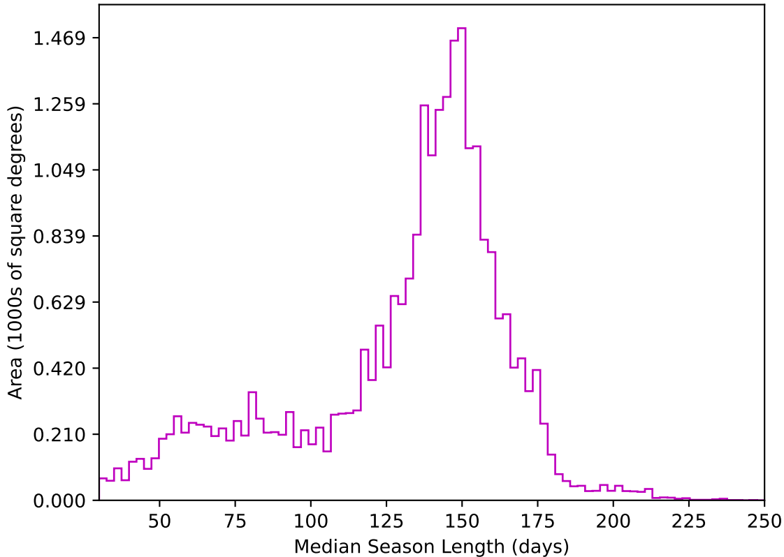
too_combined_no_nss_s10.0_v3.4_10yrs All sky z band: Median Season Length
