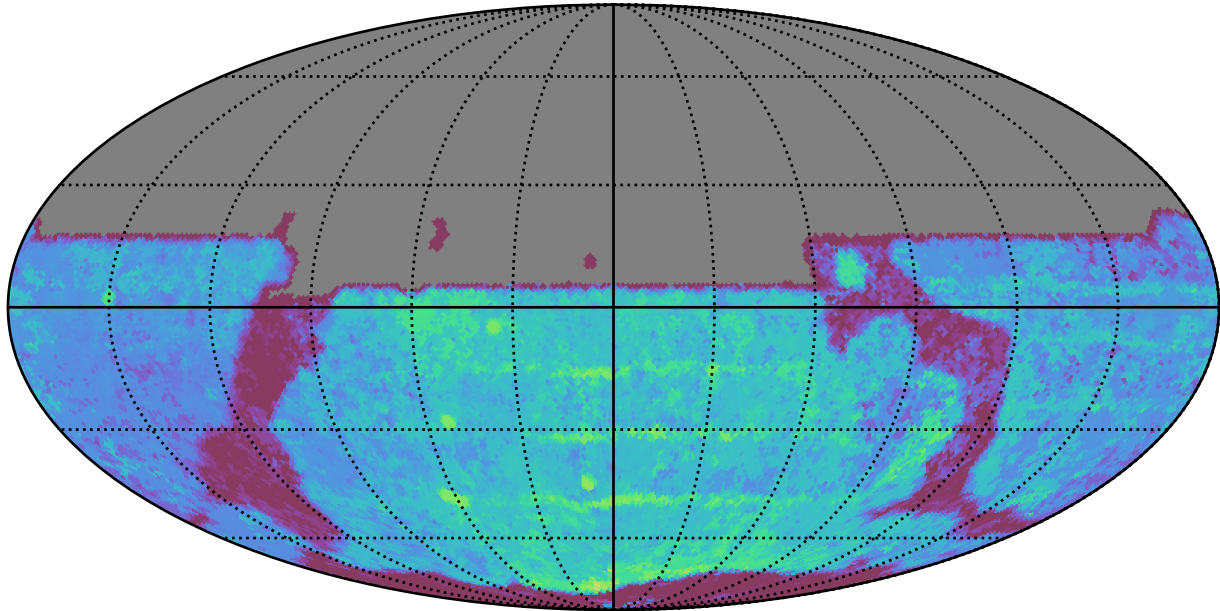
too_combined_no_nss_s10.0_v3.4_10yrs All sky y band: Median Season Length
