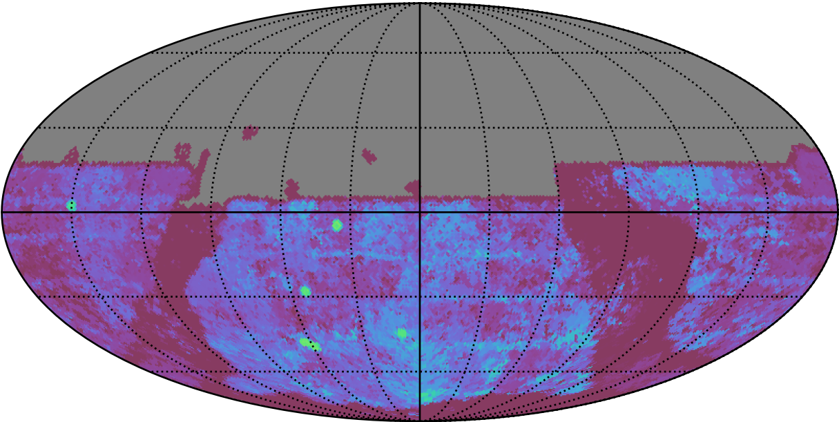
too_combined_no_nss_s10.0_v3.4_10yrs All sky u band: Median Season Length
