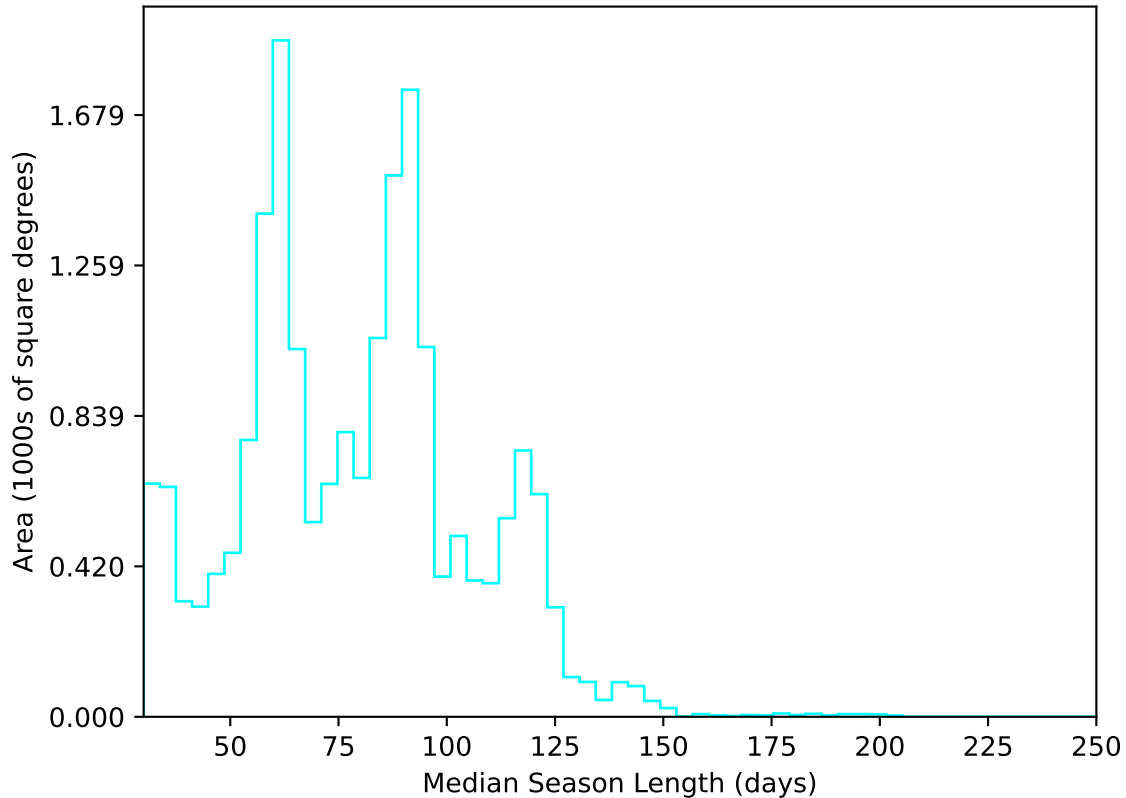
too_combined_no_nss_s10.0_v3.4_10yrs All sky u band: Median Season Length
