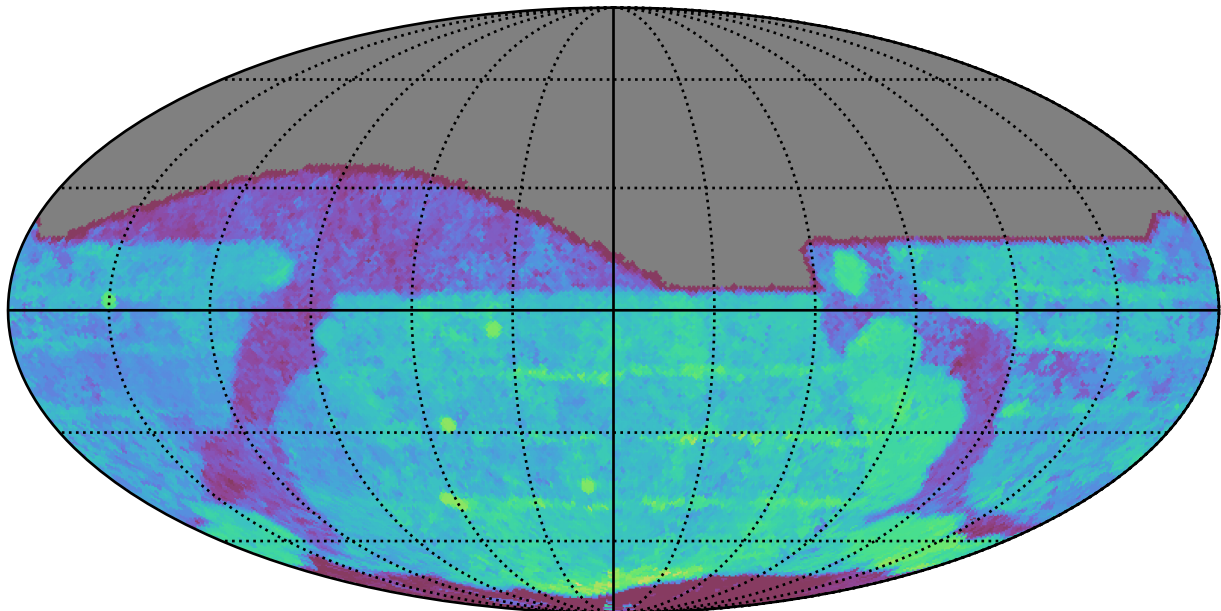
too_combined_no_nss_s10.0_v3.4_10yrs All sky r band: Median Season Length
