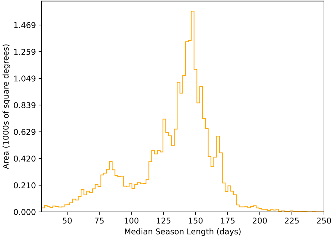
too_combined_no_nss_s10.0_v3.4_10yrs All sky r band: Median Season Length
