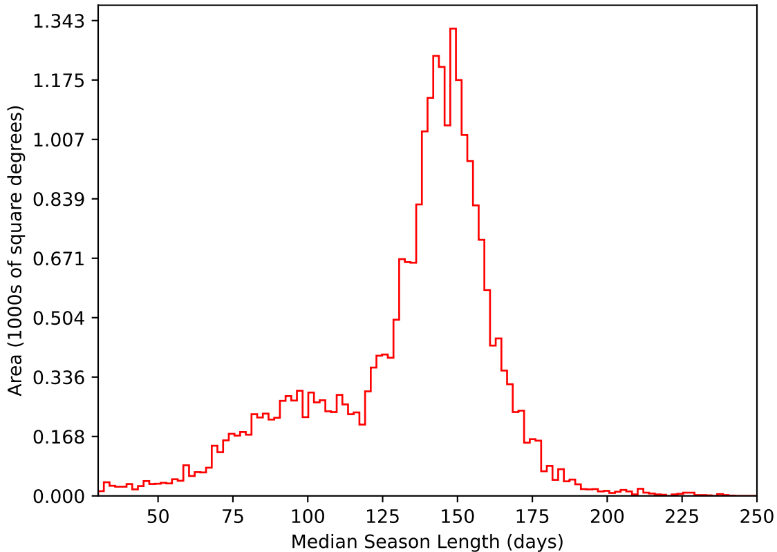
too_combined_no_nss_s10.0_v3.4_10yrs All sky i band: Median Season Length
