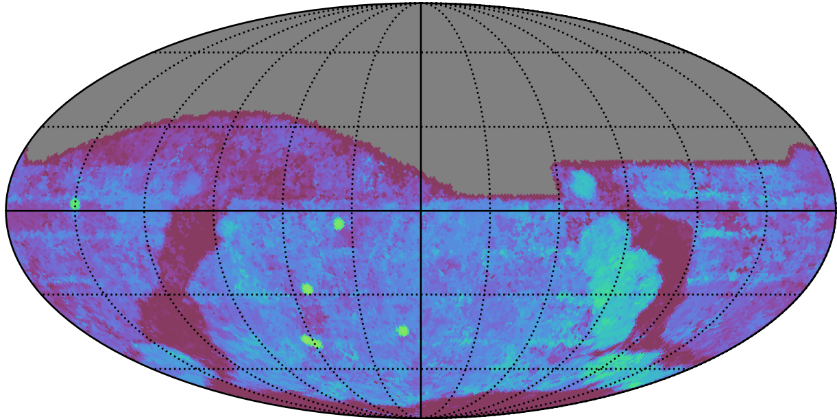
too_combined_no_nss_s10.0_v3.4_10yrs All sky g band: Median Season Length
