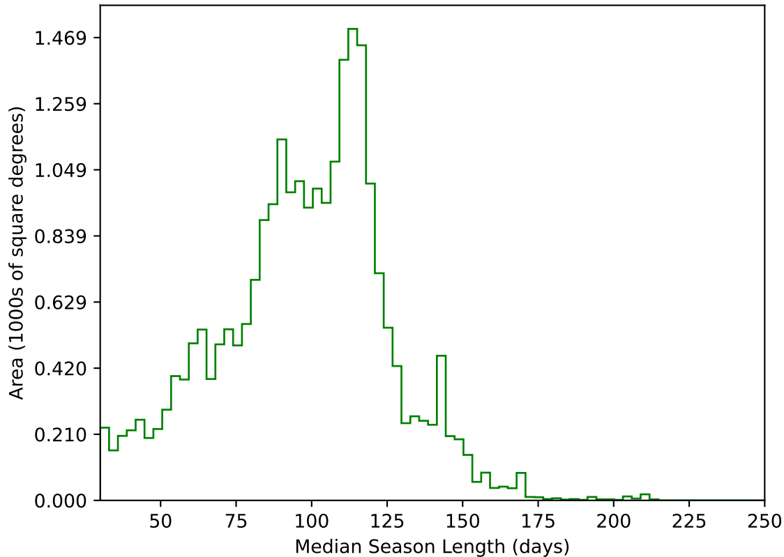
too_combined_no_nss_s10.0_v3.4_10yrs All sky g band: Median Season Length
