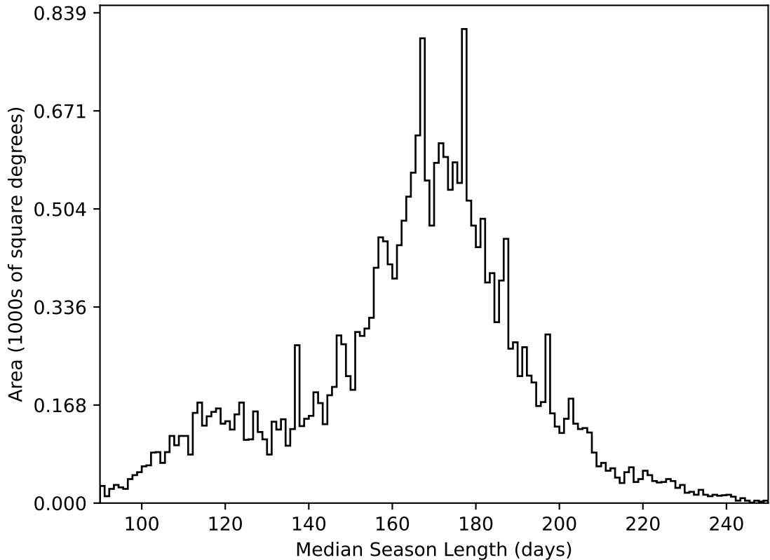
too_combined_no_nss_s10.0_v3.4_10yrs All sky all bands: Median Season Length
