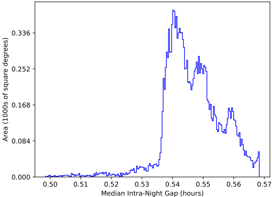
too_combined_no_nss_s10.0_v3.4_10yrs WFD: Median Intra-Night Gap
