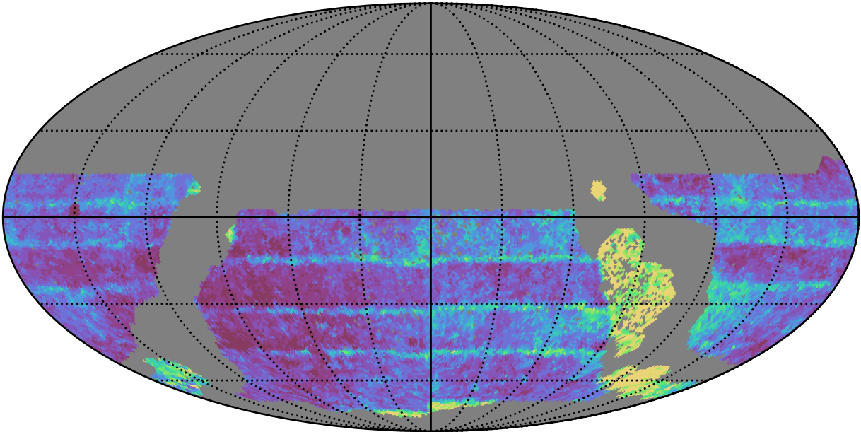
too_combined_no_nss_s10.0_v3.4_10yrs WFD z band: Median Inter-Night Gap
