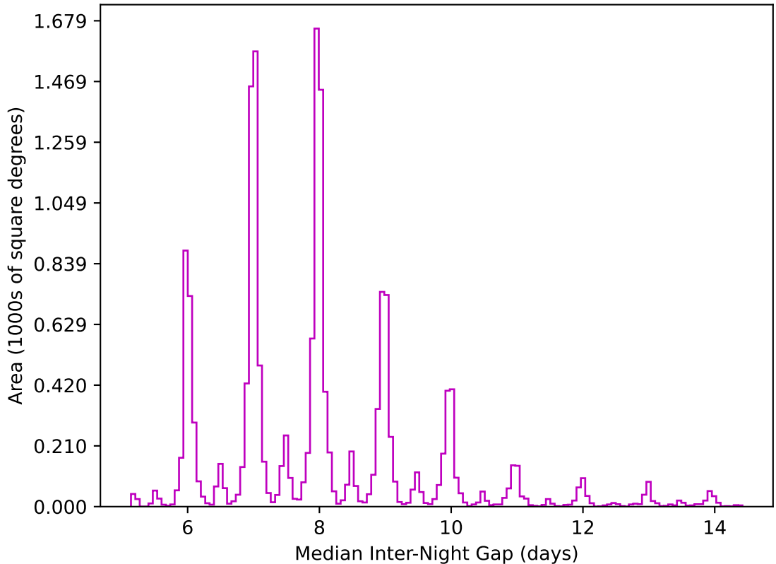
too_combined_no_nss_s10.0_v3.4_10yrs WFD z band: Median Inter-Night Gap
