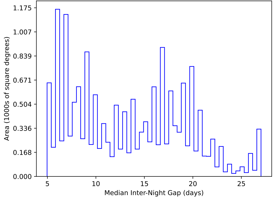
too_combined_no_nss_s10.0_v3.4_10yrs WFD y band: Median Inter-Night Gap
