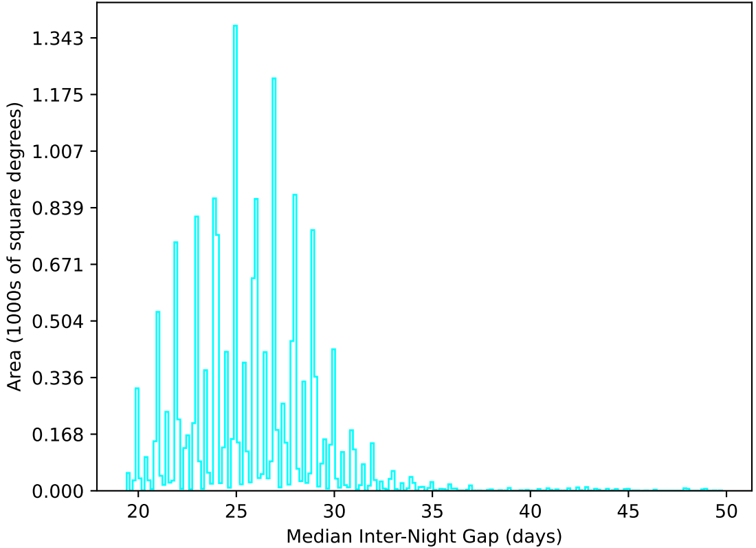
too_combined_no_nss_s10.0_v3.4_10yrs WFD u band: Median Inter-Night Gap
