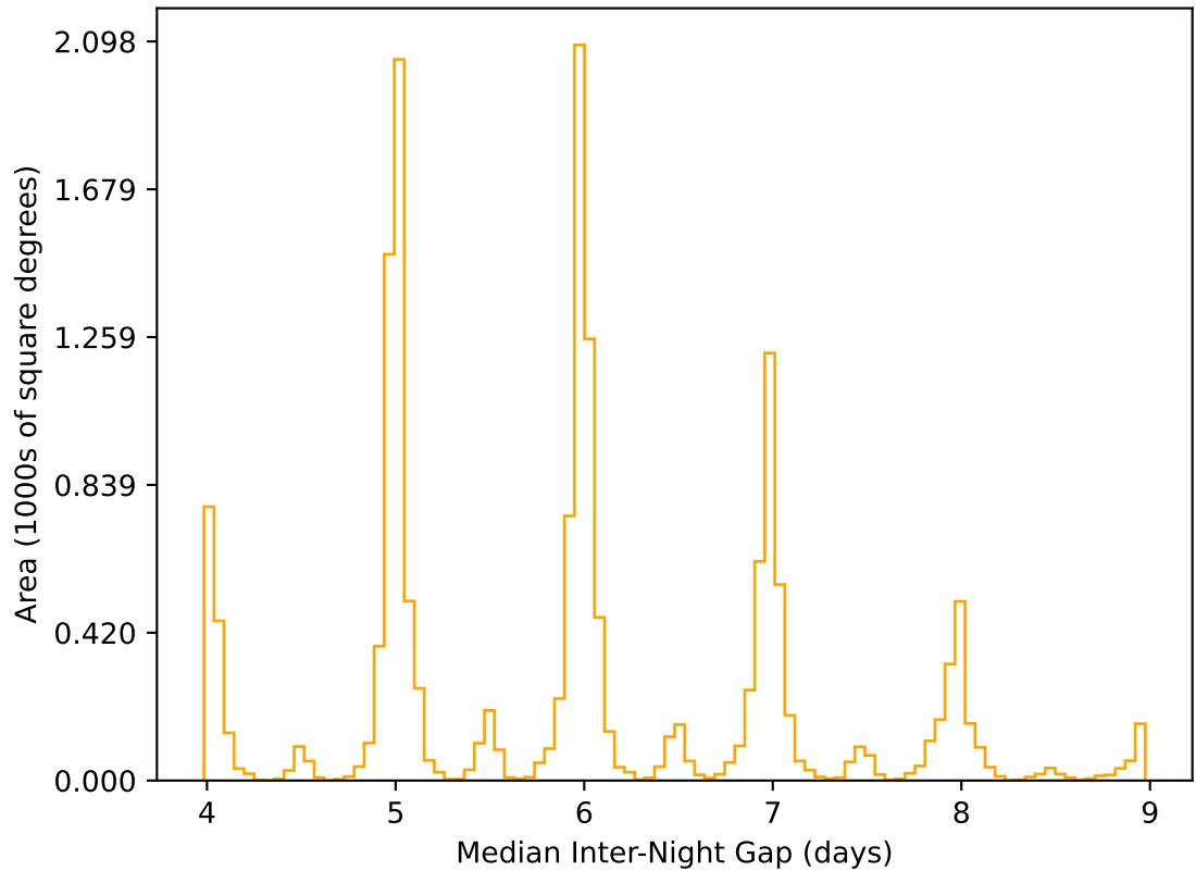
too_combined_no_nss_s10.0_v3.4_10yrs WFD r band: Median Inter-Night Gap
