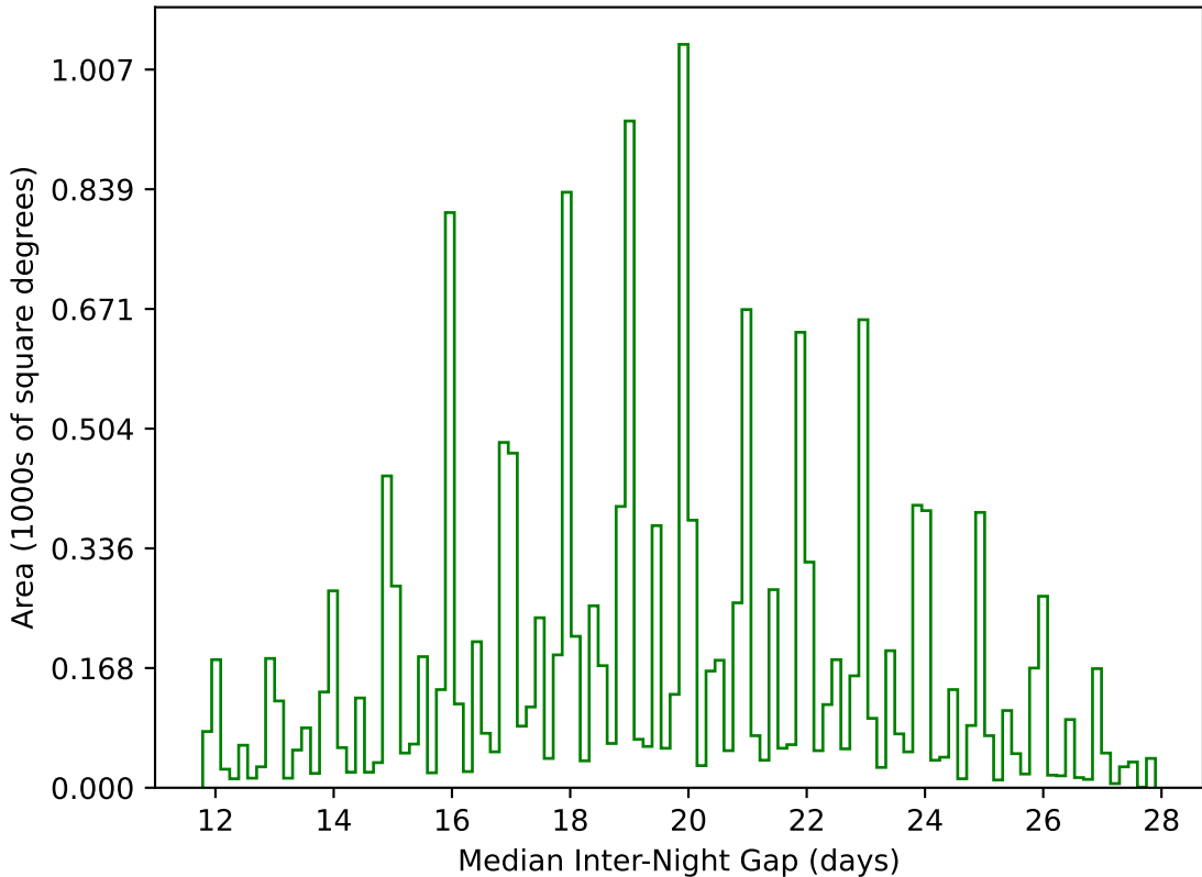
too_combined_no_nss_s10.0_v3.4_10yrs WFD g band: Median Inter-Night Gap
