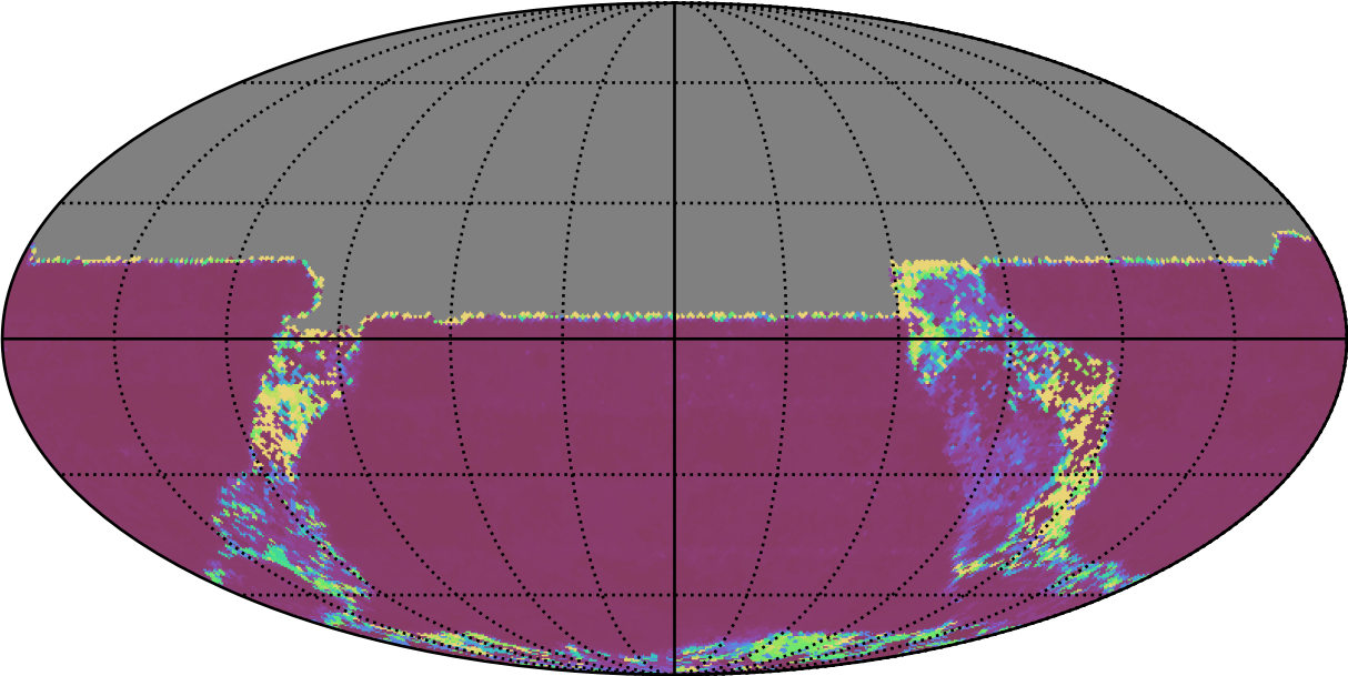
too_combined_no_nss_s10.0_v3.4_10yrs All sky u band: Median Inter-Night Gap
