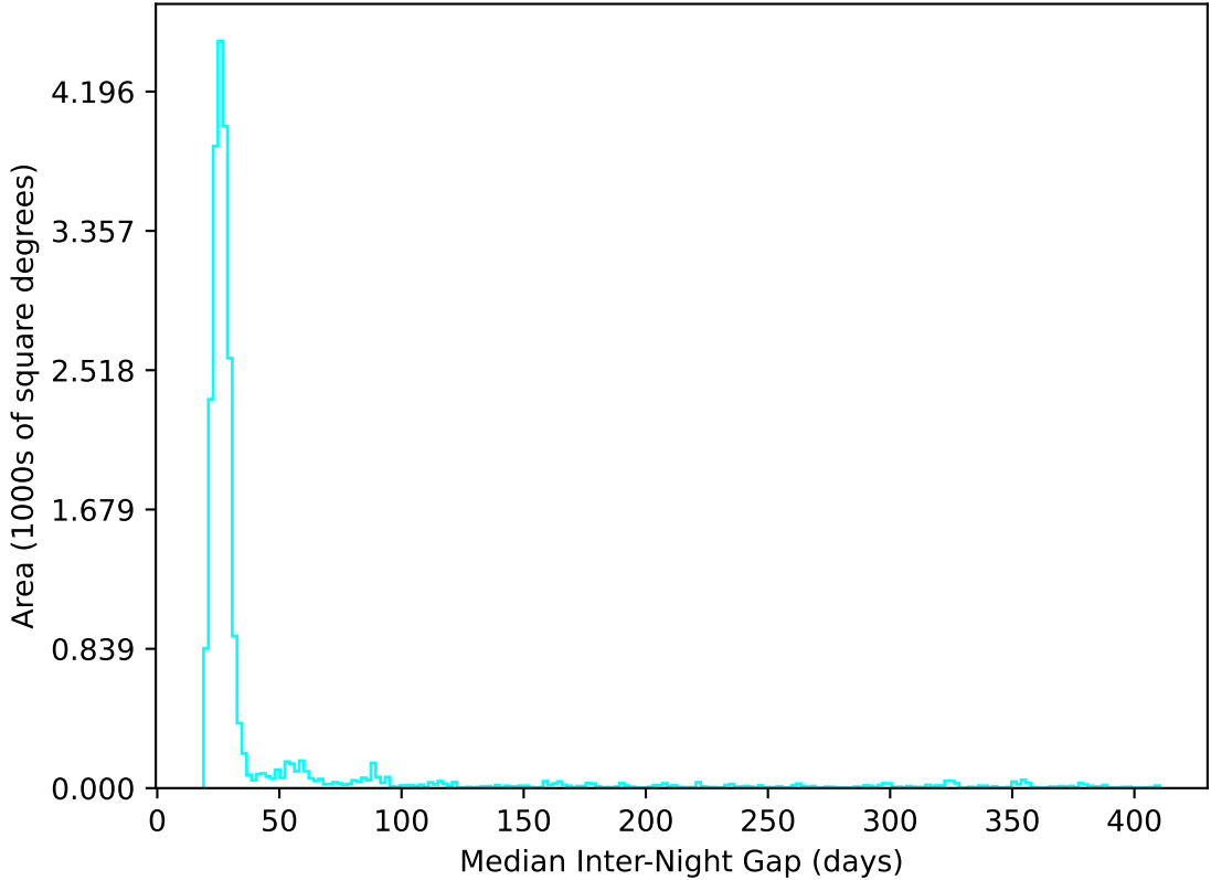
too_combined_no_nss_s10.0_v3.4_10yrs All sky u band: Median Inter-Night Gap
