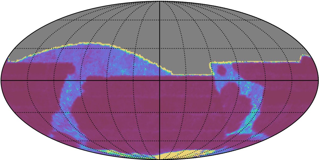
too_combined_no_nss_s10.0_v3.4_10yrs All sky r band: Median Inter-Night Gap
