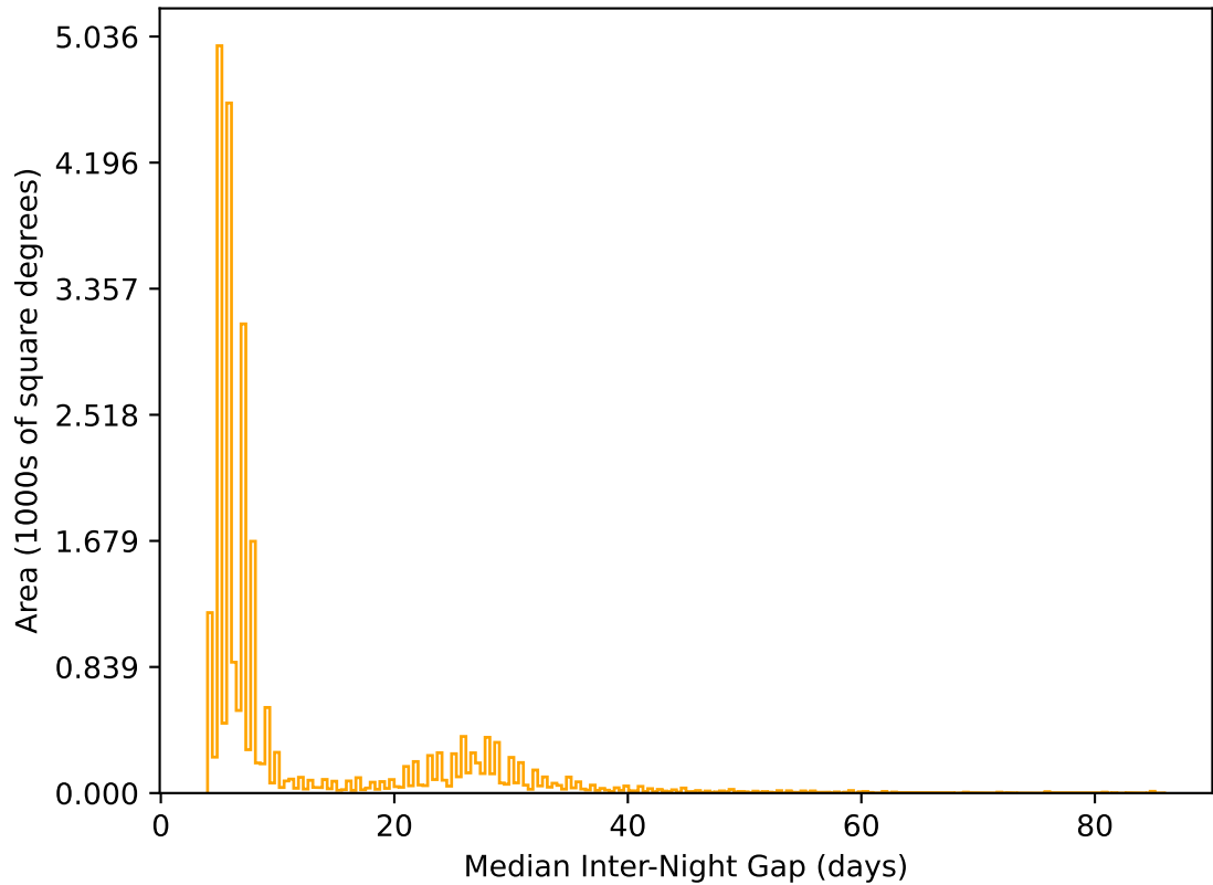
too_combined_no_nss_s10.0_v3.4_10yrs All sky r band: Median Inter-Night Gap
