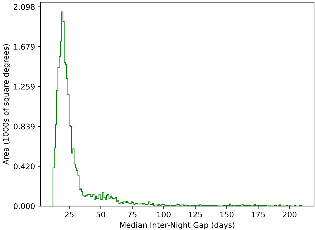
too_combined_no_nss_s10.0_v3.4_10yrs All sky g band: Median Inter-Night Gap
