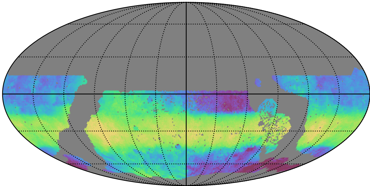
too_combined_no_nss_s10.0_v3.4_10yrs WFD z band: Median HA
