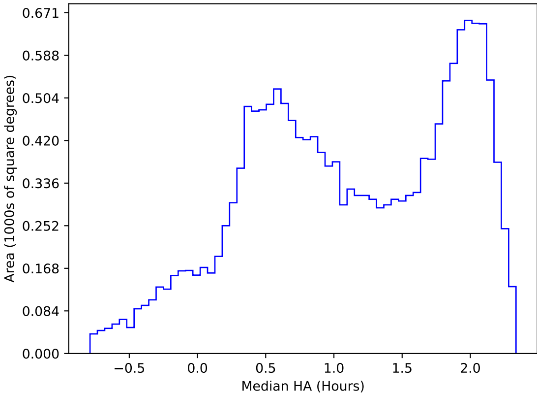
too_combined_no_nss_s10.0_v3.4_10yrs WFD z band: Median HA
