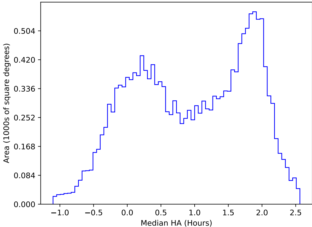
too_combined_no_nss_s10.0_v3.4_10yrs WFD u band: Median HA
