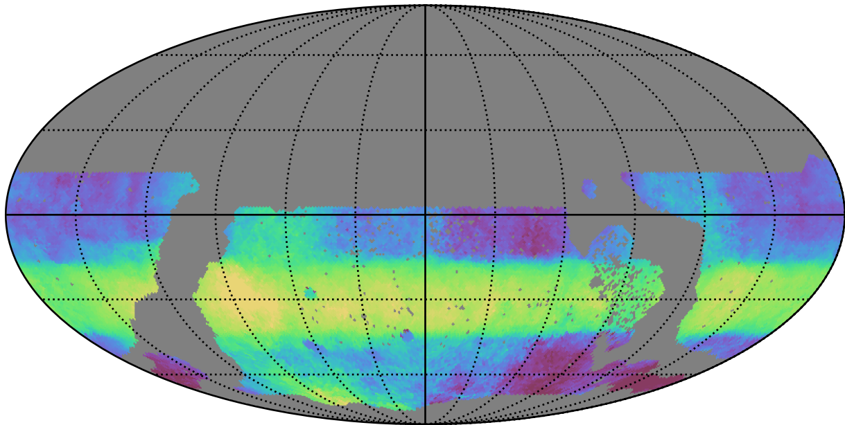
too_combined_no_nss_s10.0_v3.4_10yrs WFD r band: Median HA
