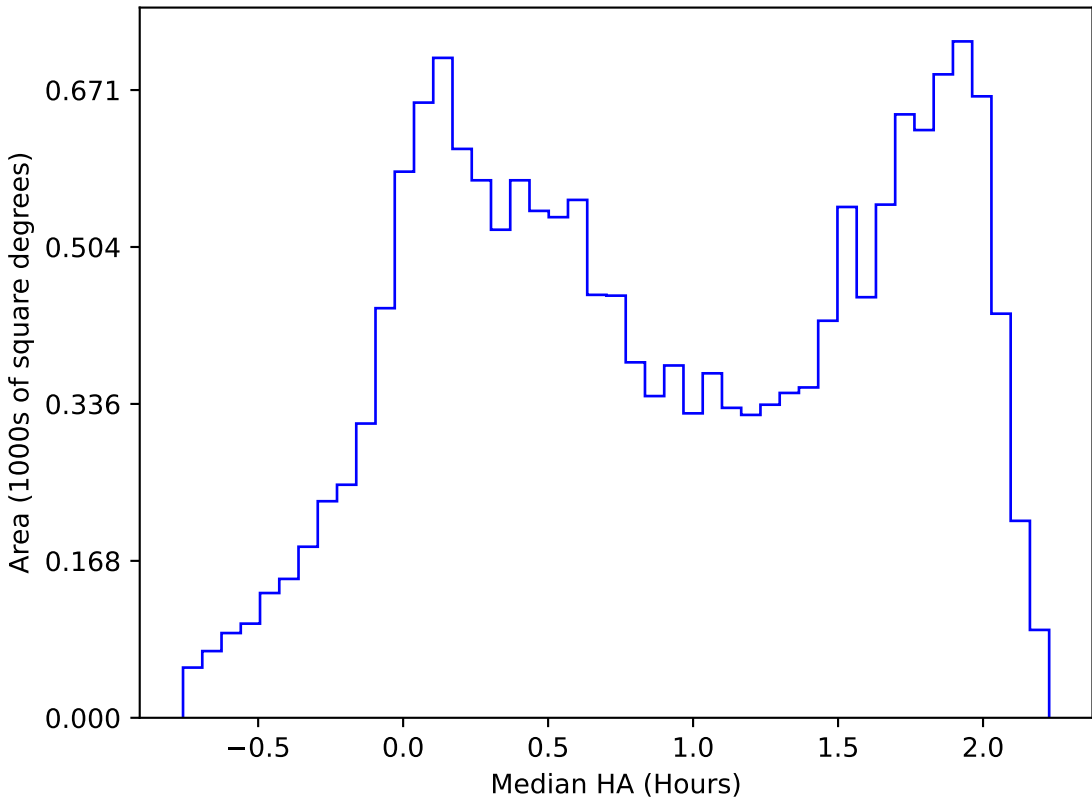
too_combined_no_nss_s10.0_v3.4_10yrs WFD r band: Median HA
