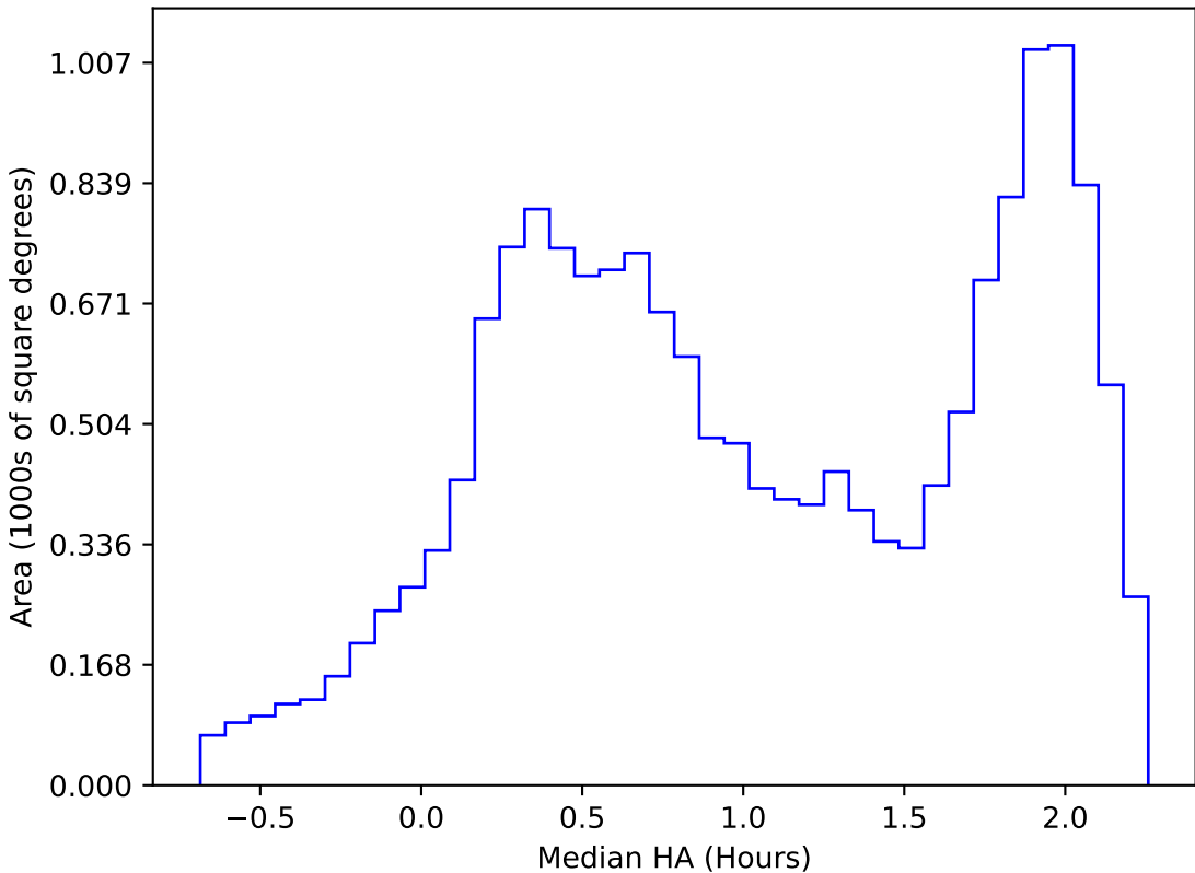
too_combined_no_nss_s10.0_v3.4_10yrs WFD i band: Median HA
