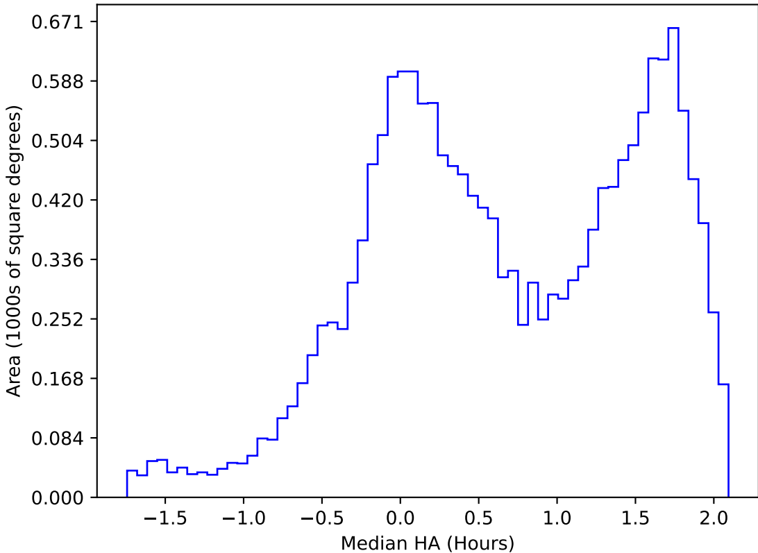
too_combined_no_nss_s10.0_v3.4_10yrs WFD g band: Median HA
