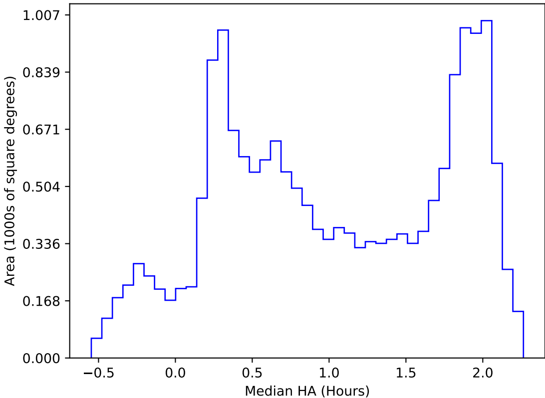
too_combined_no_nss_s10.0_v3.4_10yrs WFD all bands: Median HA
