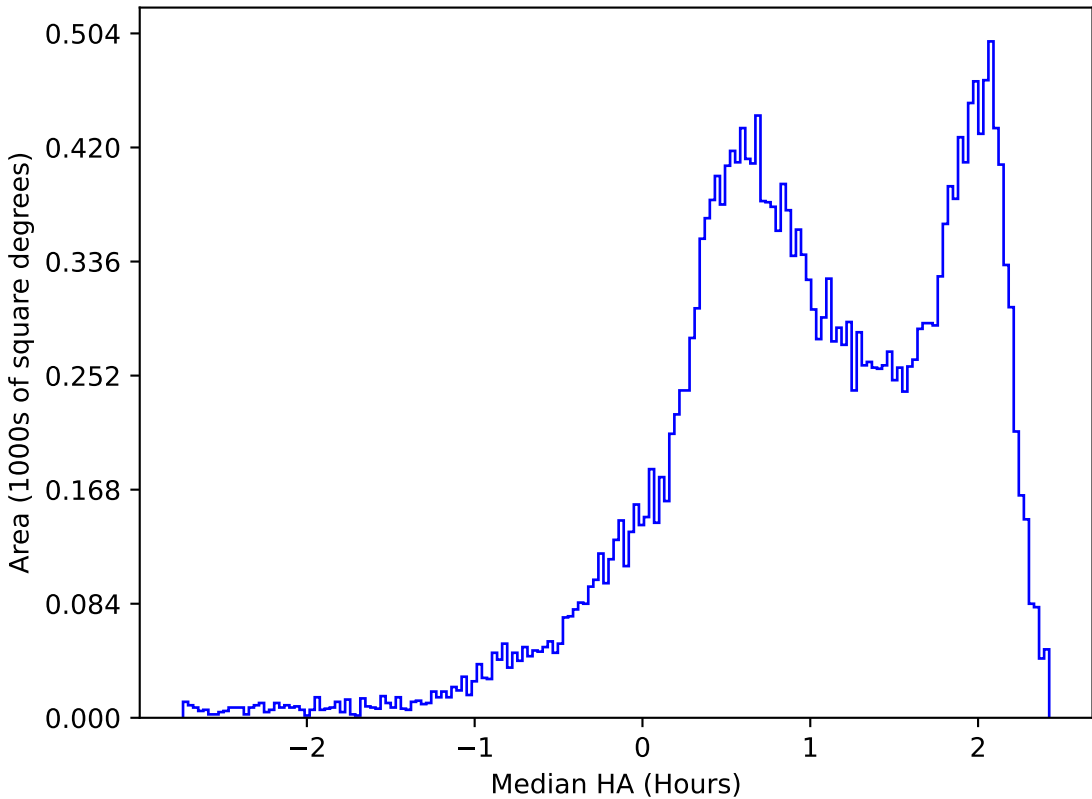
too_combined_no_nss_s10.0_v3.4_10yrs All sky z band: Median HA
