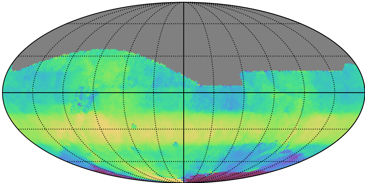
too_combined_no_nss_s10.0_v3.4_10yrs All sky r band: Median HA
