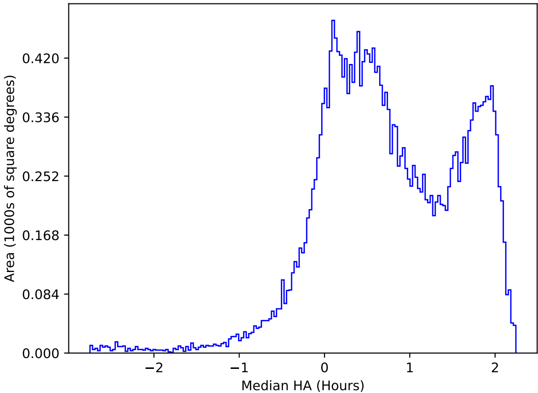
too_combined_no_nss_s10.0_v3.4_10yrs All sky r band: Median HA
