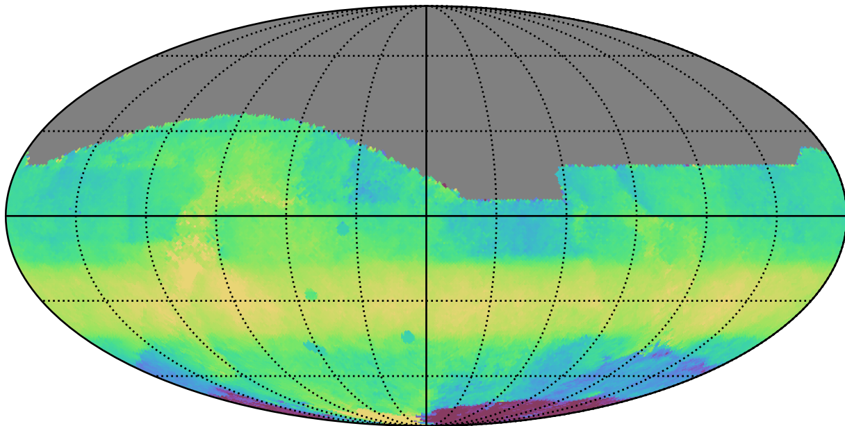
too_combined_no_nss_s10.0_v3.4_10yrs All sky i band: Median HA
