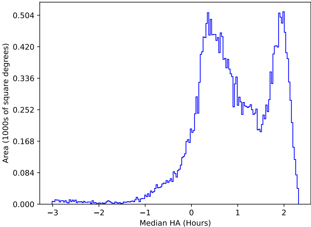
too_combined_no_nss_s10.0_v3.4_10yrs All sky i band: Median HA
