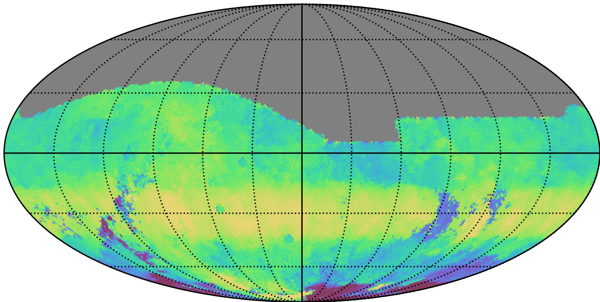
too_combined_no_nss_s10.0_v3.4_10yrs All sky g band: Median HA
