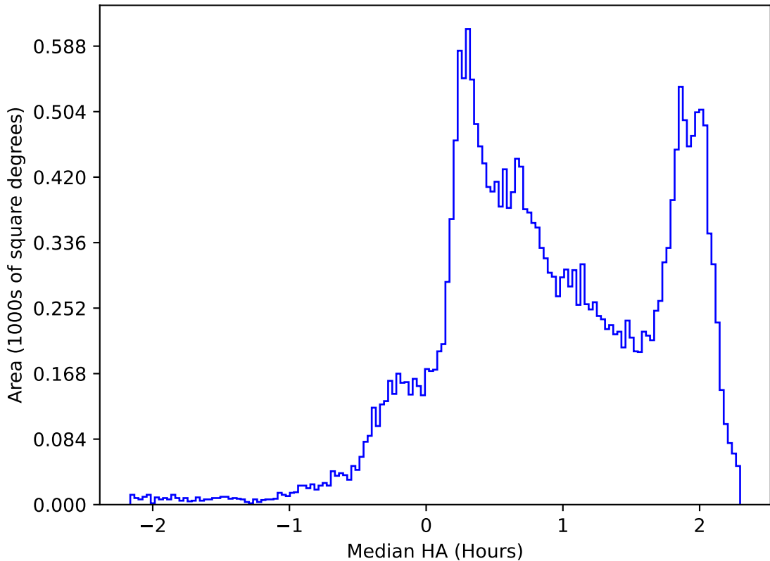
too_combined_no_nss_s10.0_v3.4_10yrs All sky all bands: Median HA
