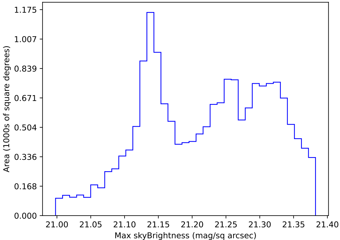
too_combined_no_nss_s10.0_v3.4_10yrs WFD r band: Max skyBrightness
