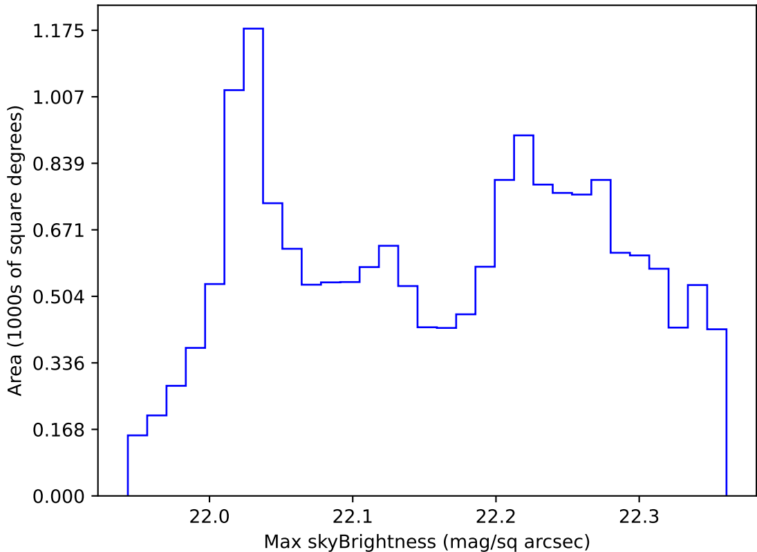
too_combined_no_nss_s10.0_v3.4_10yrs WFD g band: Max skyBrightness
