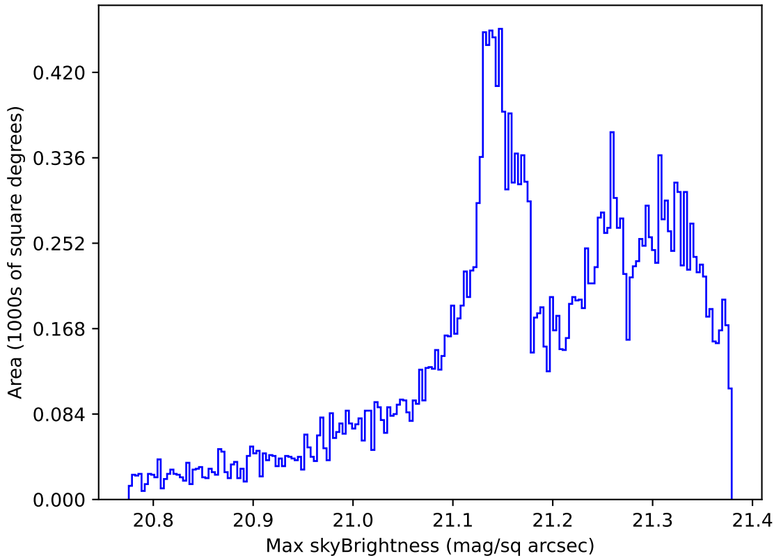
too_combined_no_nss_s10.0_v3.4_10yrs All sky r band: Max skyBrightness
