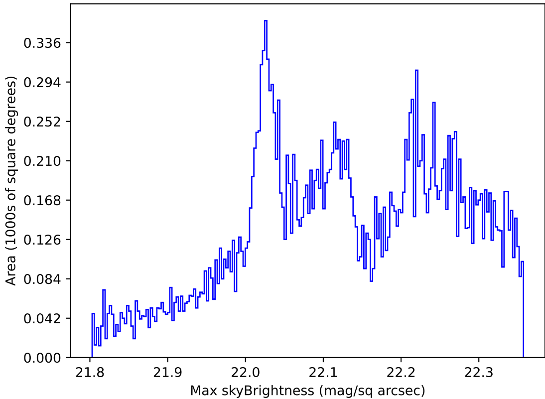
too_combined_no_nss_s10.0_v3.4_10yrs All sky g band: Max skyBrightness
