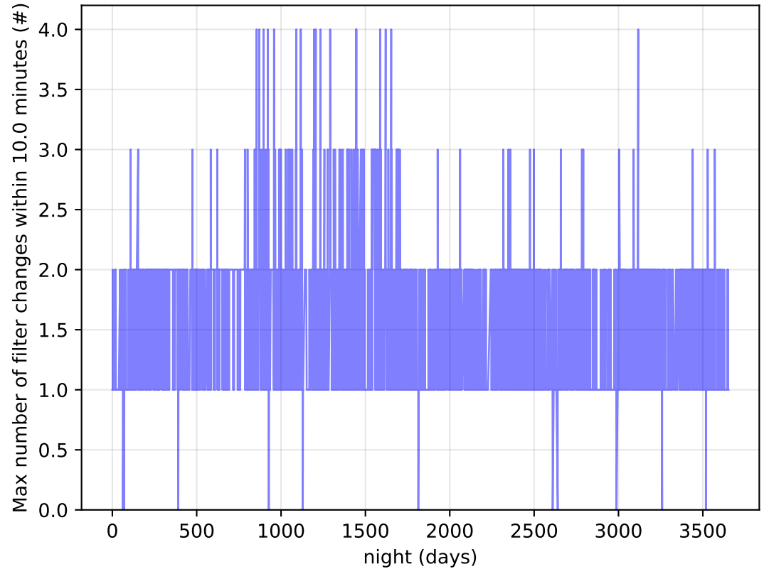
too_combined_no_nss_s10.0_v3.4_10yrs Per Night: Max number of filter changes within 10.0 minutes
