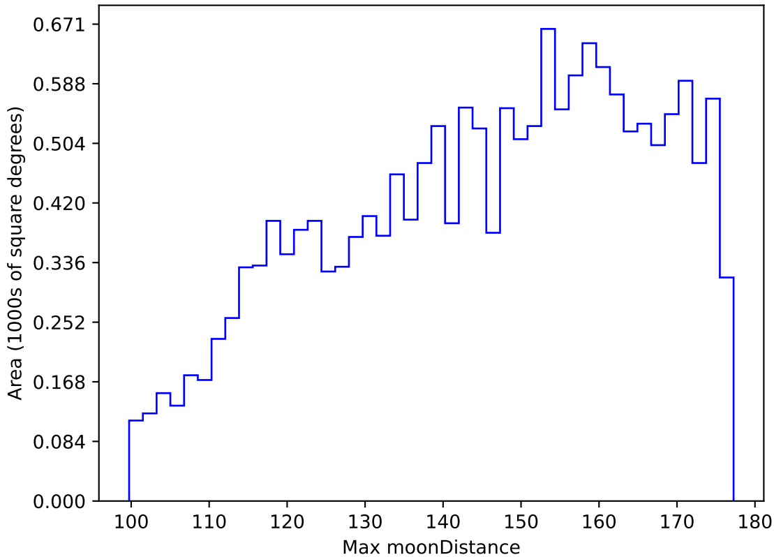
too_combined_no_nss_s10.0_v3.4_10yrs WFD y band: Max moonDistance
