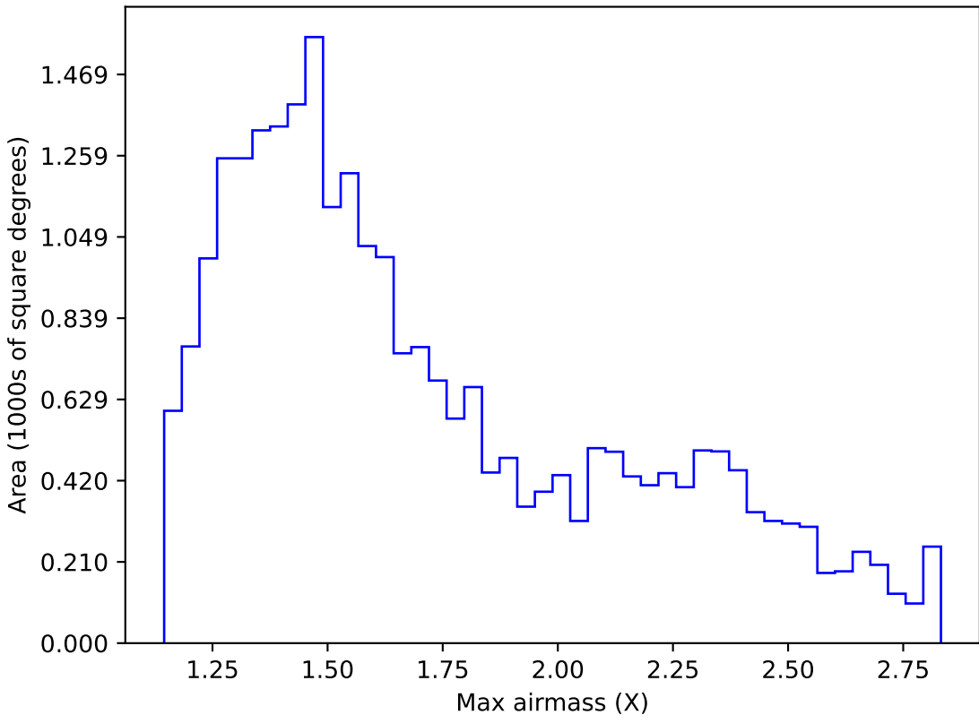
too_combined_no_nss_s10.0_v3.4_10yrs Yr 1 z band: Max airmass
