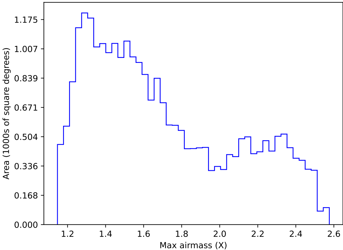
too_combined_no_nss_s10.0_v3.4_10yrs Yr 1 r band: Max airmass
