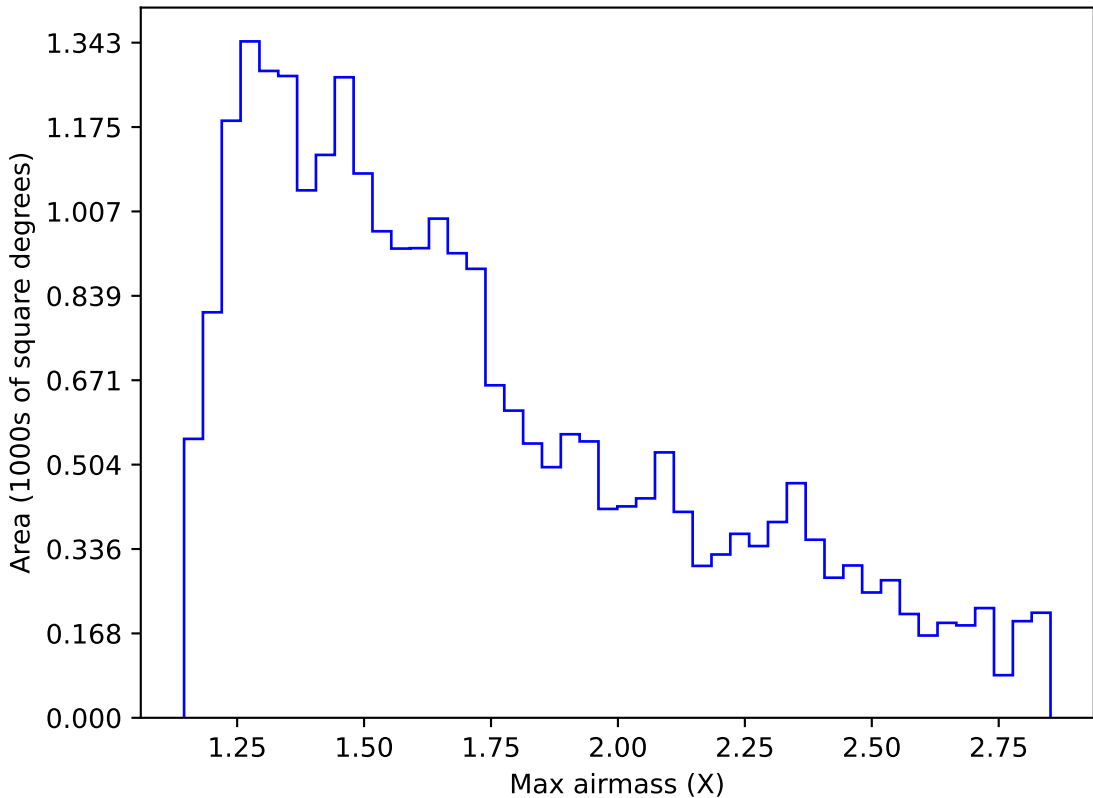
too_combined_no_nss_s10.0_v3.4_10yrs Yr 1 i band: Max airmass
