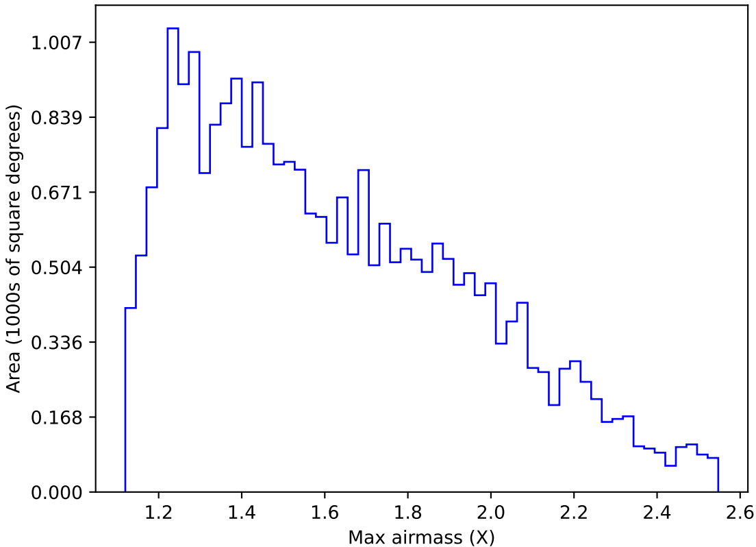
too_combined_no_nss_s10.0_v3.4_10yrs Yr 1 g band: Max airmass
