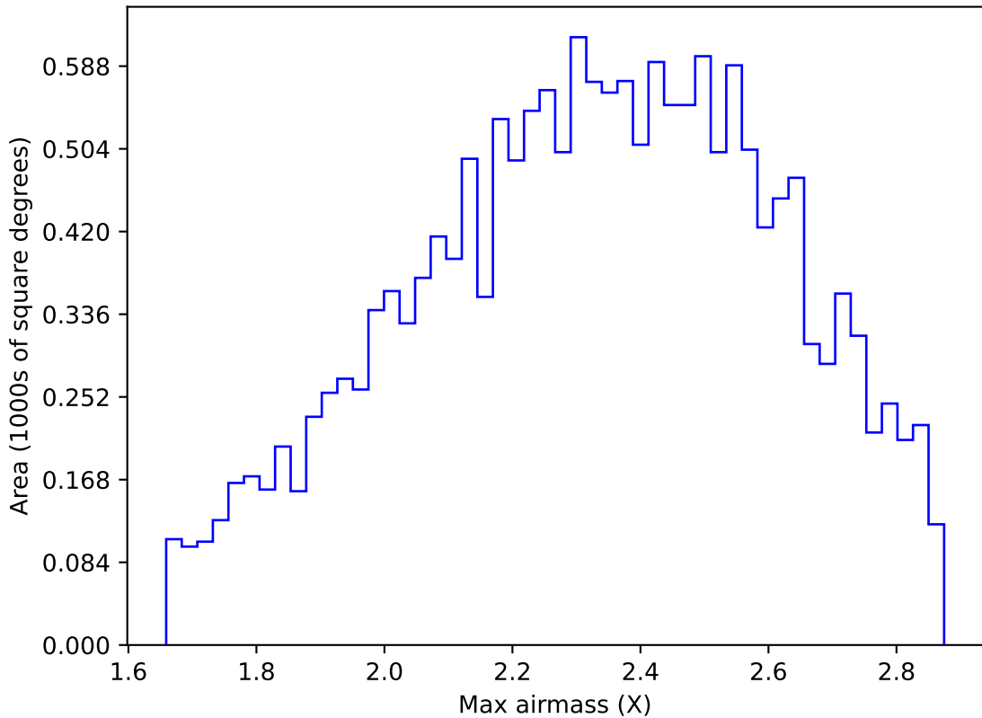
too_combined_no_nss_s10.0_v3.4_10yrs WFD y band: Max airmass
