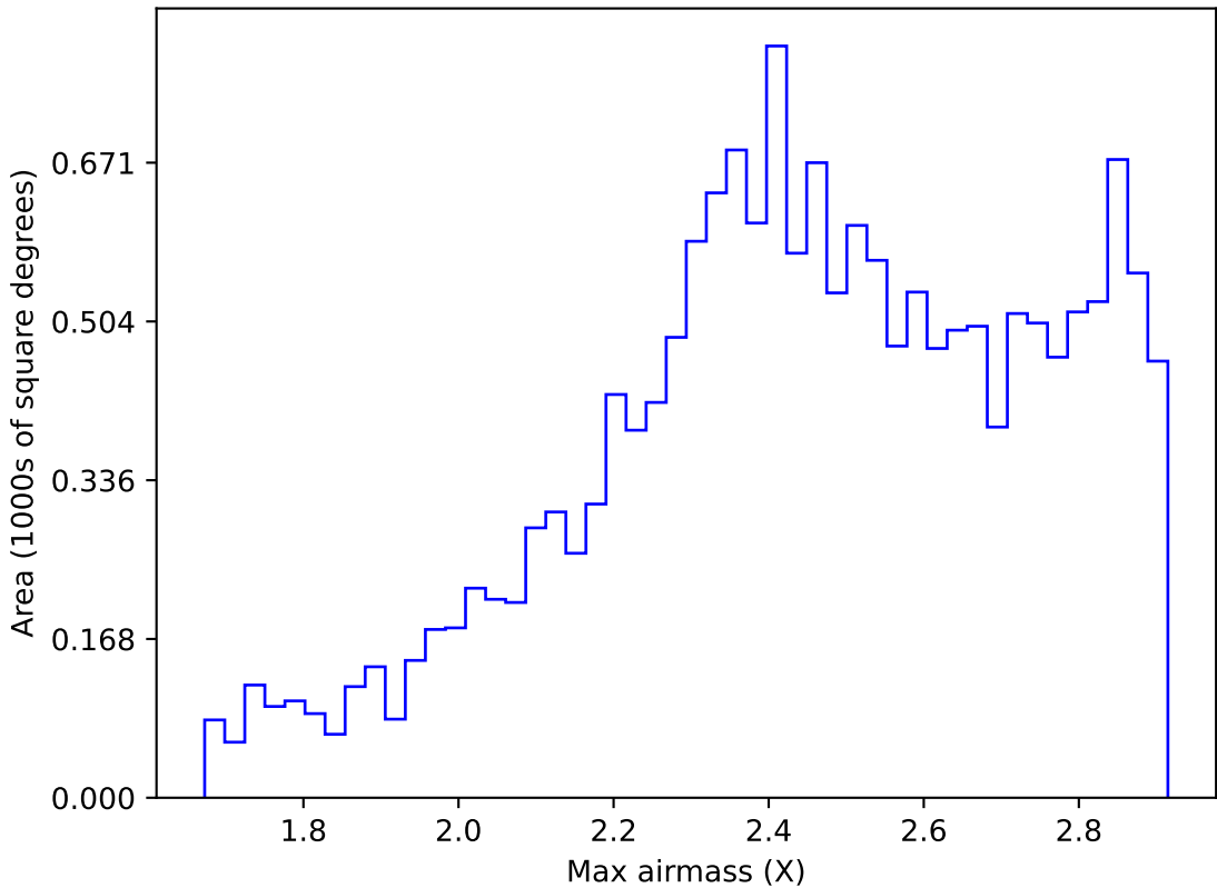
too_combined_no_nss_s10.0_v3.4_10yrs WFD i band: Max airmass
